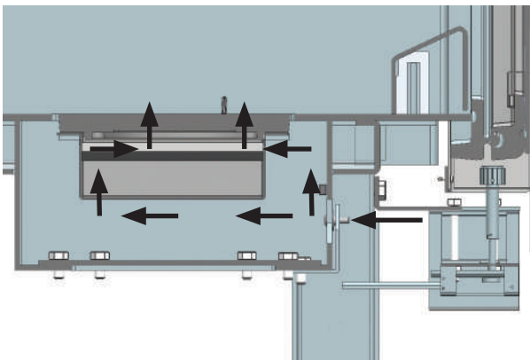
FIG. 16 - Primary air valve
