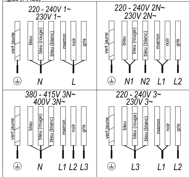
Fig.2b (7 FILS)
