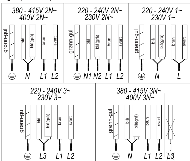
Fig.2a (5 KABLER)
