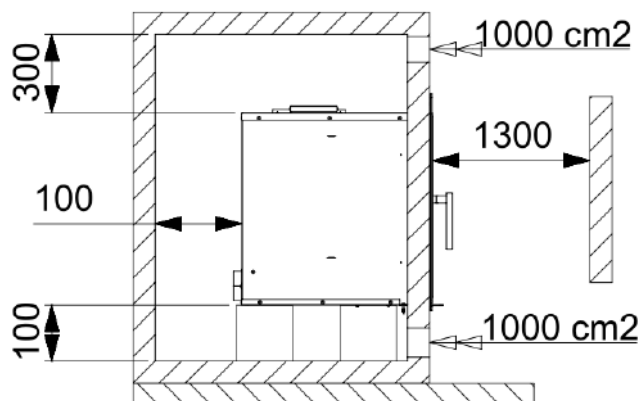
Minimum safety distances of combustibles materials "N" and "N CT" version
